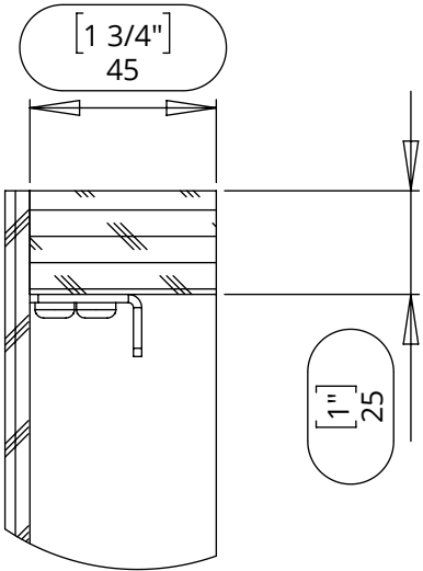
DETAIL Q SCALE 1 : 2
