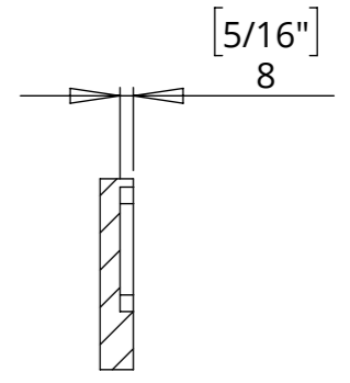
SECTION G-G
