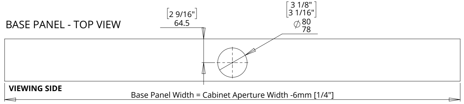
BOX ENCLOSURE BASE PANEL - TOP VIEW
