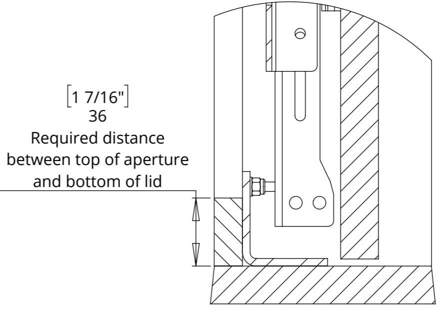
DETAIL O
