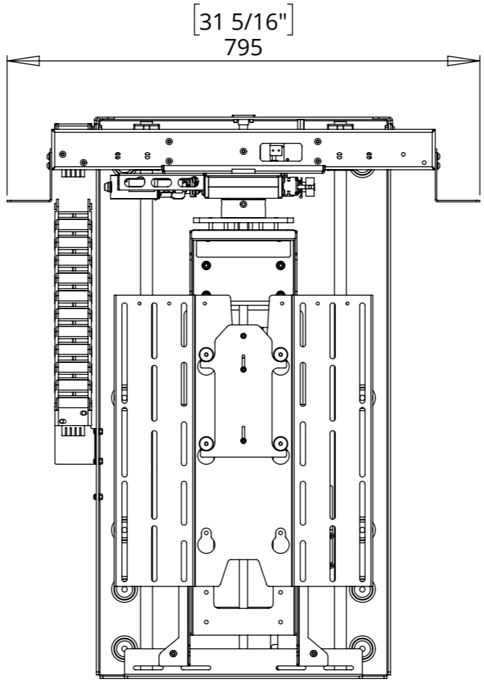
MECHANISM - UP POSITION
