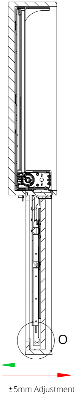
SECTION N-N
