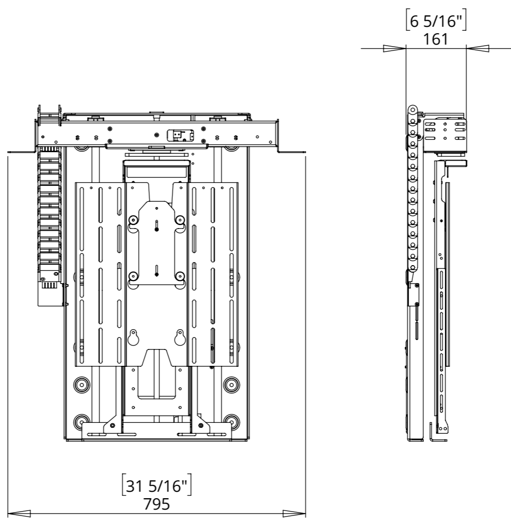
MECHANISM - UP POSITION
