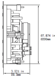
MOUNTING DEPTH/ MINIMUM CUTOUT
