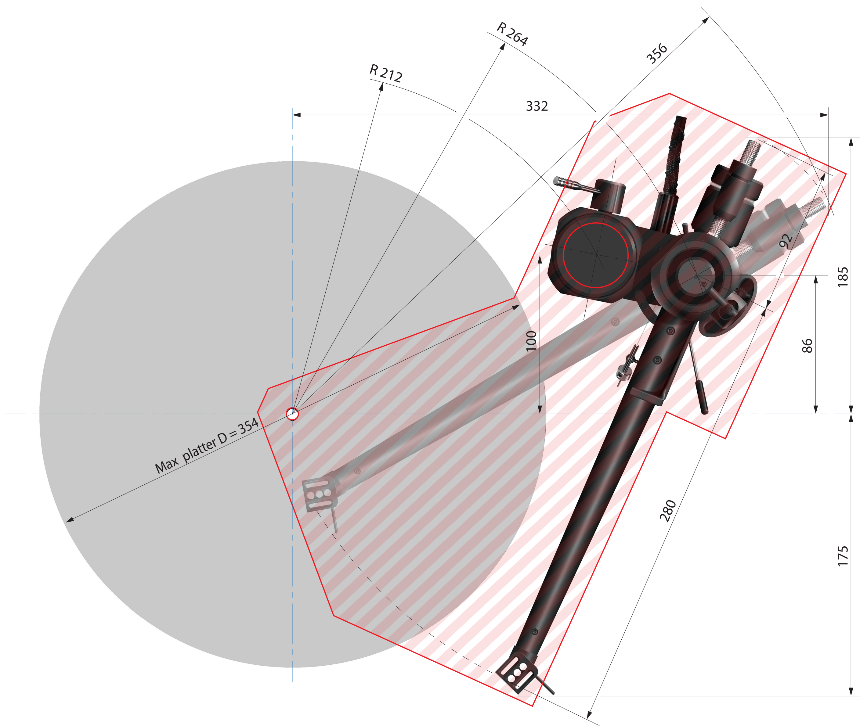
KUZMA 4Point Tonearm Top view
