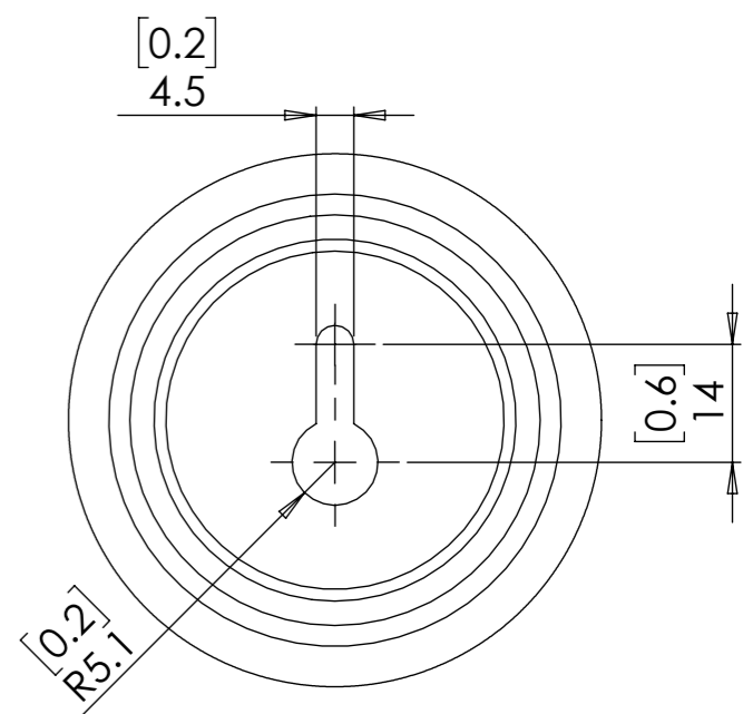
VIEW B
