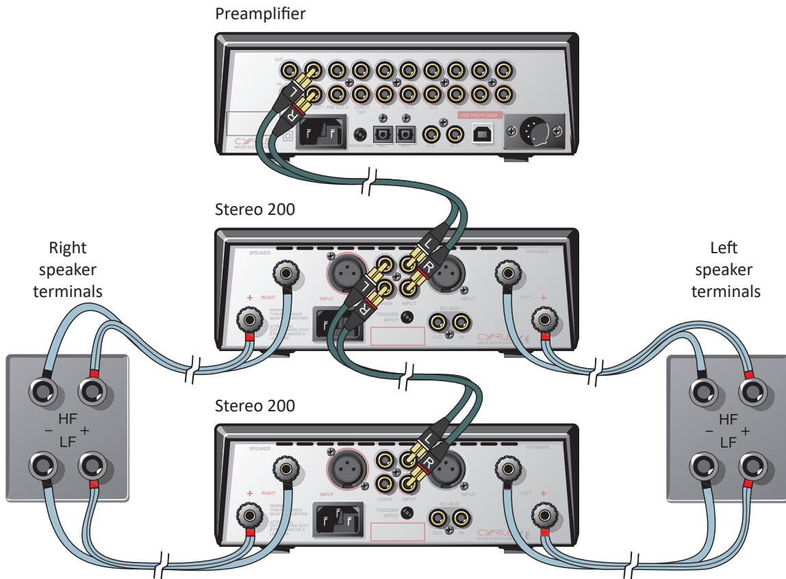
Chain output and bi-amplified speaker connection
