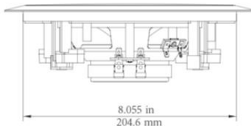
MINIMUM CUTOUT
