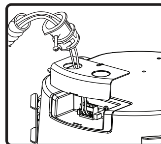
4. Run signal wires through conduit connector, then through cover plate. Connect to Euroblock connector.
