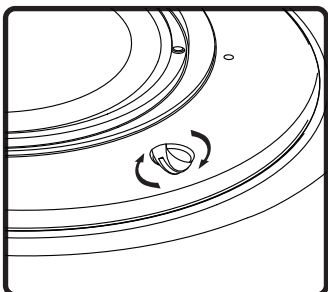
8. Select the tap position by adjusting rotary switch to desired high impedance value or voice coil direct mode.
