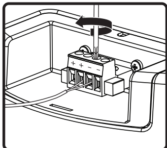
5. Connect to Euroblock connector. Two + and two - connectors are provided for daisy chaining.
