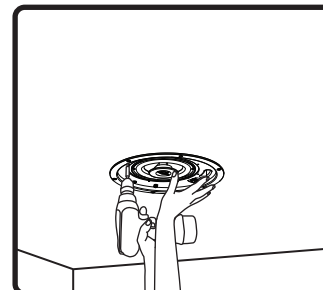
7. Insert speaker into mounting hole. Screw down both bolts on the baffle face to actuate the mounting wings. Firmly secure both bolts – do not over-tighten.
