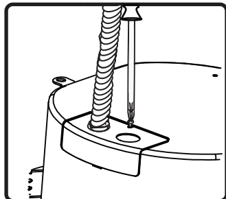
6. Tighten screw on terminal plate, and push conduit connector into knockout.
