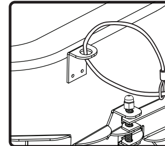
8. If required, a sheet-metal tab located on the rear panel of the speaker serves as a secondary point of attachment (cable not included).
