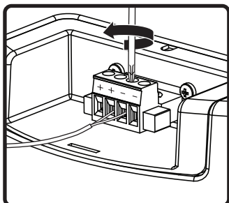
5. Connect to Euroblock connector. Two + and two - connectors are provided for daisy chaining.
