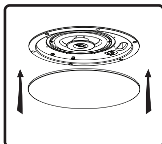
11. Place grille onto baffle. (The grille is held in place by magnets in the baffle.)
