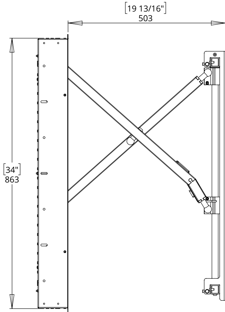
MAX EXTENSION
