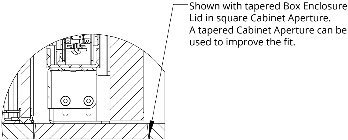
DETAIL F
