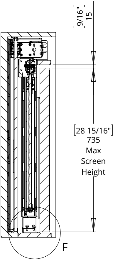
SECTION E-E
