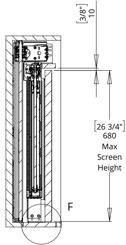
SECTION E-E
